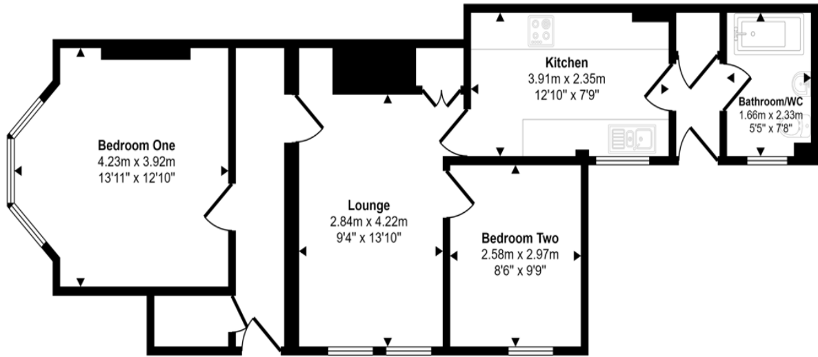
Floorplan
