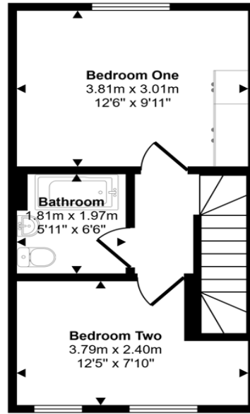
First Floor Approx 29 sq m / 312 sq ft
