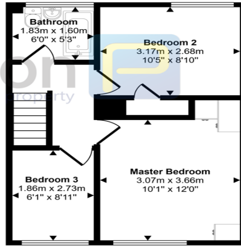
First Floor Approx 36 sq m / 390 sq ft
